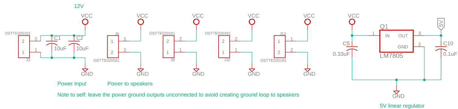
5V linear regulator
